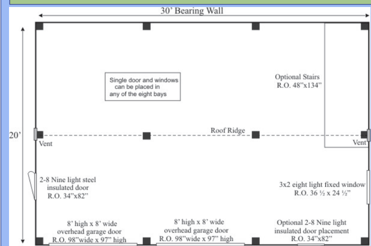
Option A Floor Plan
